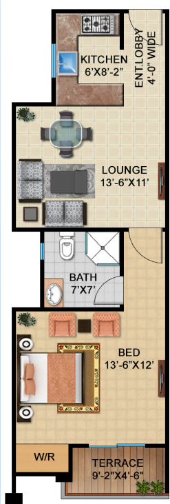
TYPE-B (4TH & 6TH FLOOR) TOTAL AREA 682 SFT.
