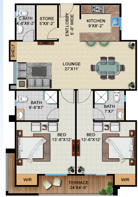
TYPE-A (3RD TO 7TH, 9TH & 11TH FLOOR) TOTAL AREA 1694 SFT.
