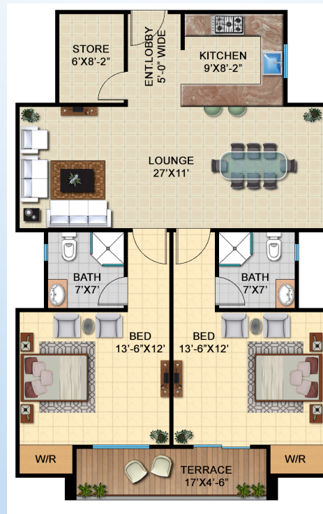
TYPE-A1 (3RD, 5TH & 7TH FLOOR) TOTAL AREA 1363 SFT.
