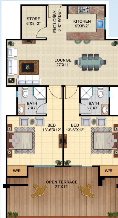
TYPE-A1 (3RD FLOOR) TOTAL AREA 1582 SFT.
